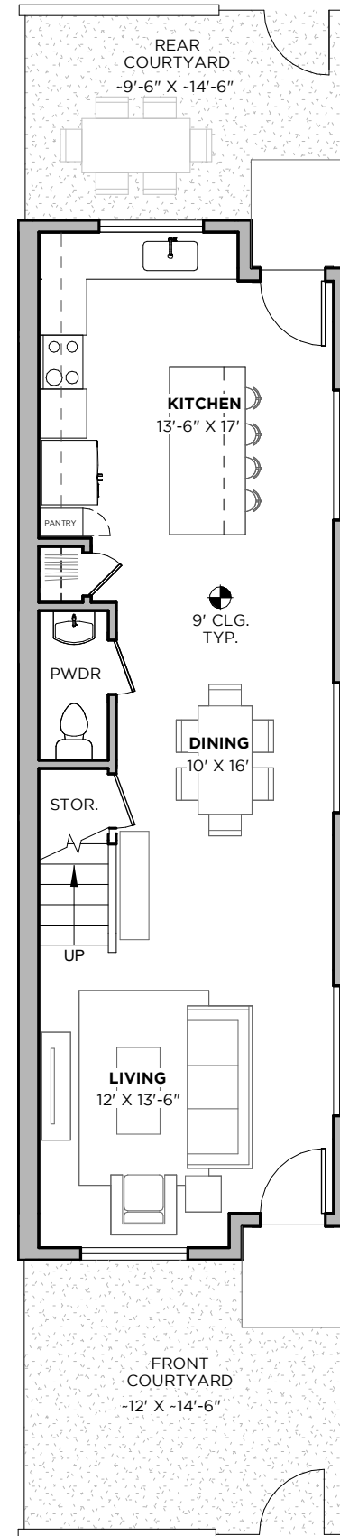
First Floor
