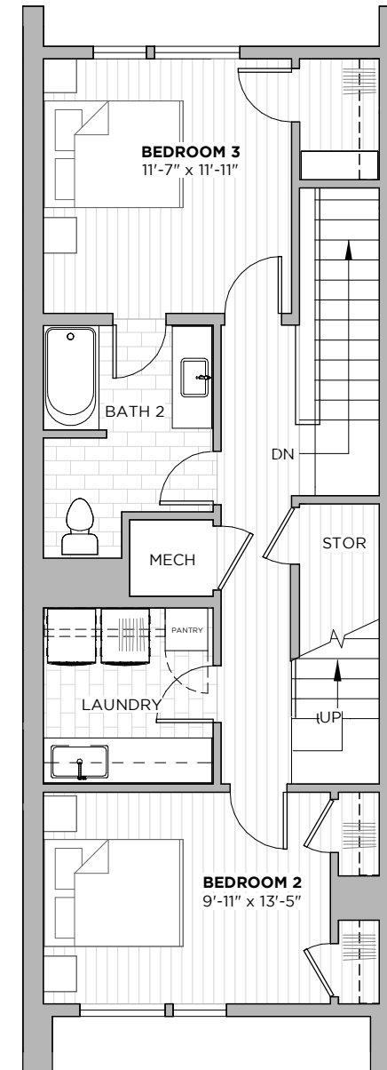
SECOND FLOOR
