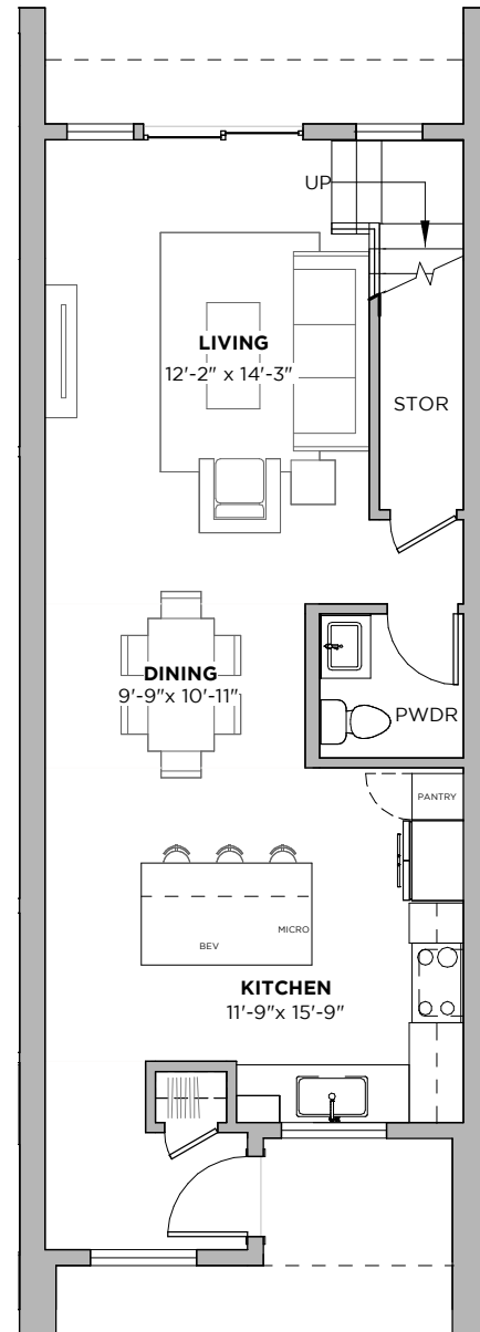
FIRST FLOOR
