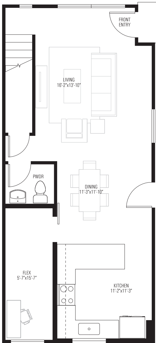
GROUND
